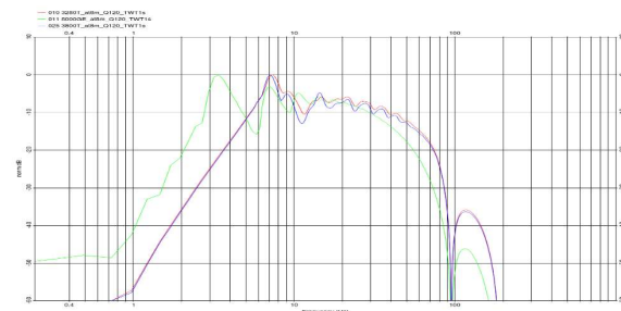
Figure 1: Gemini (green) source signature amplitude spectrum compared to a conventional marine source arrays (red and blue), with Earth filter applied.
