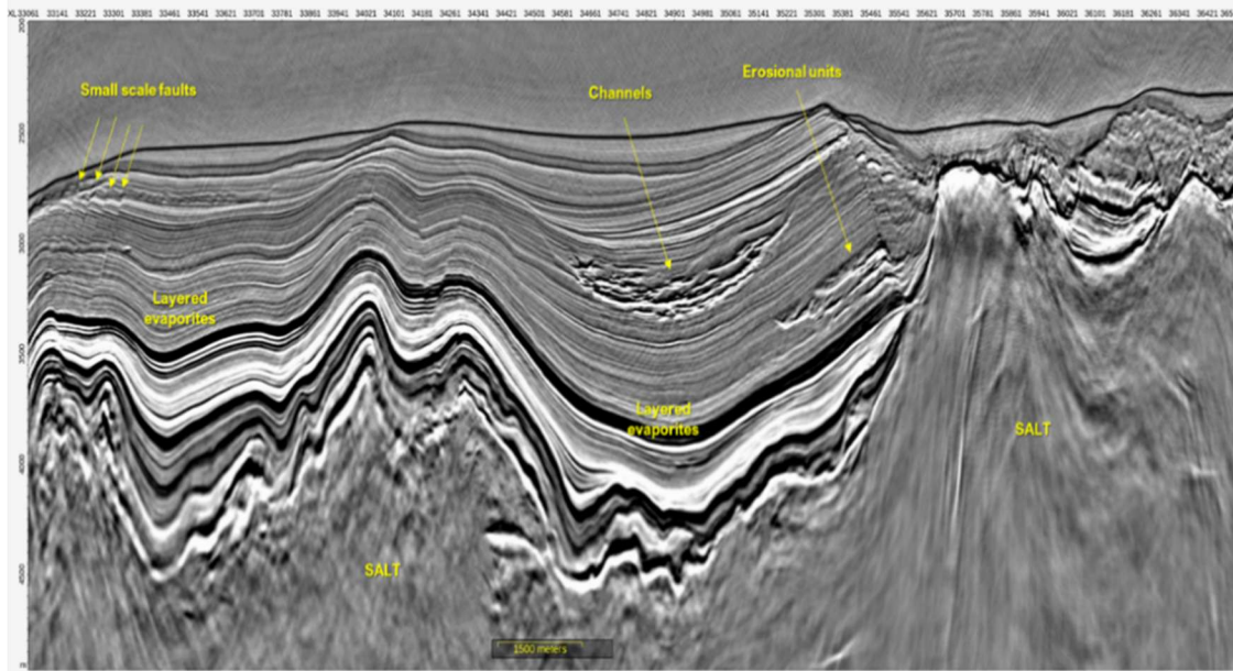
Figure 6: Fast-track PSDM stack from Angola dataset showing preserved high-frequency content and interpretation of small-scale features.
