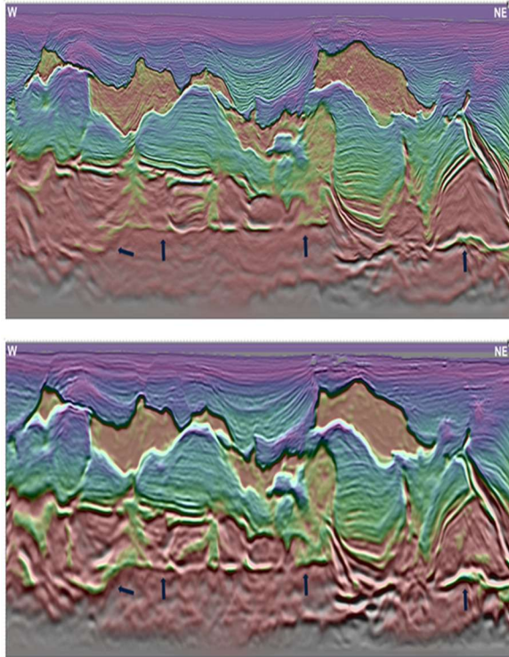
Figure 4: Arbitrary line showing elastic FWI model overlay with FWI image from conventional gun array (top) and extended-frequency source (bottom). Even at an intermediate stage of processing (6 Hz), Amendment Phase 4 show with Gemini source shows improved deep basement imaging and geologically more plausible structures, mostly because of better low frequencies.
