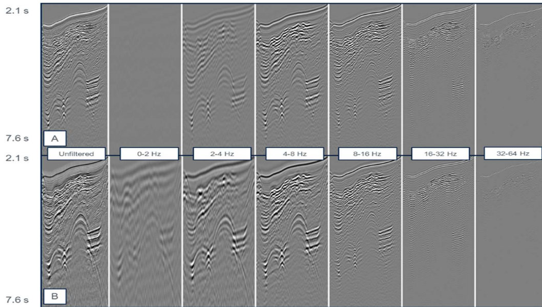
Figure 5: Octave panels from conventional (A) and extended-frequency (B) sources from the Angola streamer data. Notice the improved low-frequency content and S/N in the first two octave panels.
