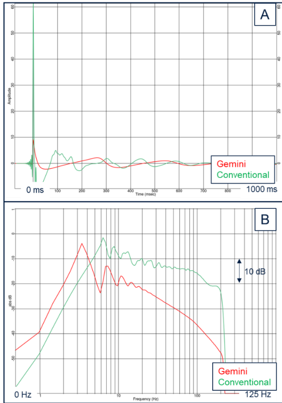
Figure 3 A): the enhanced frequency source compared to the conventional source; B): log amplitude spectra for the two wavelets shown in 3B. (Note: the conventional (legacy) source wavelet is estimated based on the acquisition vessel used).
