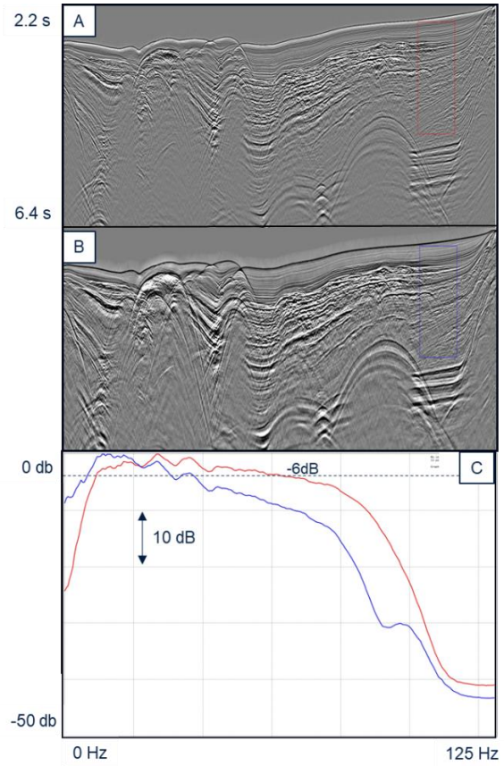
Figure 4: pre-processed stacks after regularization; A) conventional source; B) enhanced frequency source; C) Amplitude spectra
