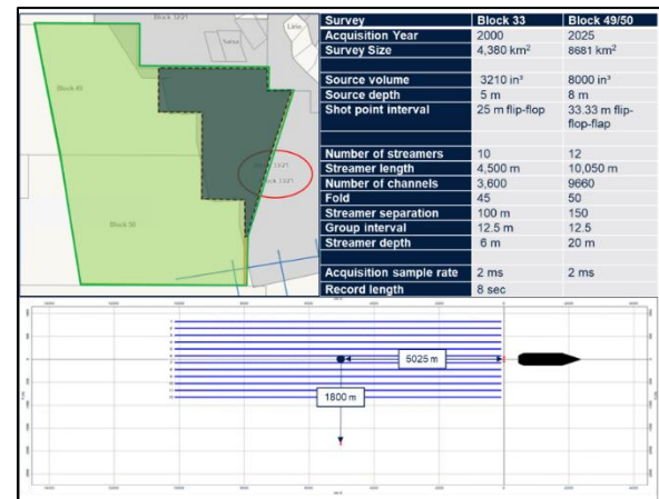
Figure 1 top: Key acquisition parameters for the new acquisition (Block 49/50) and the legacy (Block 33); bottom: vessel layout for the new acquisition.
