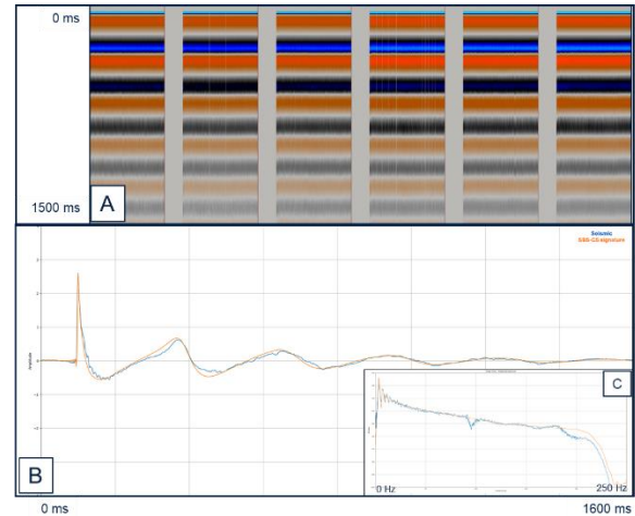
Figure 2 A): SBS-CS wavelets for both vessels; B): TX domain representation of the SBS-CS signature (orange) and a data extracted wavelet; C): amplitude spectra for the two wavelets shown in 2B.
