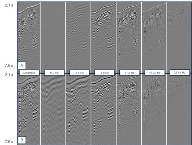
Figure 6: octave panels; A) conventional source; B) enhanced frequency source.
