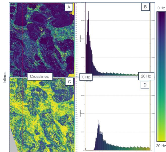
Figure 5: maps of the frequency at -6dB down. The dimensions of the map are 27 km x 31 km; A and B) map and histogram for the enhanced frequency source; C and D) map and histogram for the conventional source.
