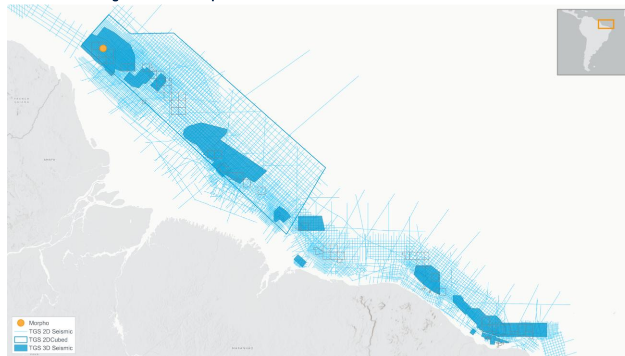
TGS data coverage over the Morpho well
