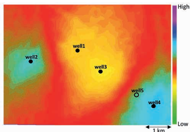
Figure 12 Horizon slice in the zone of interest for the low-frequency model generated using an inverse-distance interpolation method. (Data courtesy: Arcis Seismic Solutions, TGS, Calgary).
