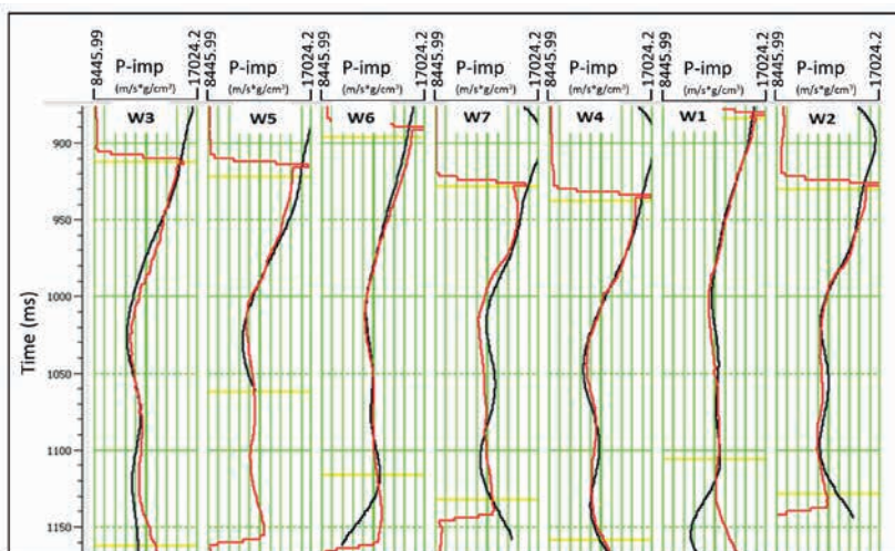
Figure 3 Match between the modelled impedance log and actual filtered impedance log using multi-attribute training network after including single well low-frequency model as one of the input. Black curve represents the filtered impedance log and red curve represents the modelled impedance curve. Analysis window is marked by yellow bar. Correlation coefficient improves significantly to 0.96.
