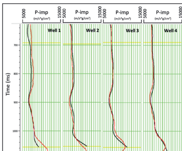
Figure 10 Validation match between the modelled impedance log and actual filtered impedance log using multi-attribute network after including a single well low-frequency model as one of the inputs. Black curve represents the filtered impedance log and red curve represents the modelled impedance curve. Analysis window is marked by yellow bar. A high correlation coefficient of 0.89 is observed.
