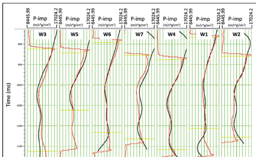
Figure 4 Validation match between the modelled impedance log and actual filtered impedance log using multi-attribute network after including a single well low-frequency model as one of the input. Black curve represents the filtered impedance log and red curve represents the modelled impedance curve. Analysis window is marked by yellow bar. A high correlation coefficient of 0.92 is observed.
