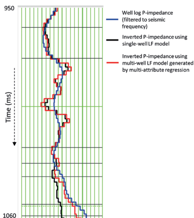
Figure 13 Match at the blind well between the actual impedance logs (blue curve), inverted impedance using single well low-frequency model (black curve) and the inverted impedance using the low-frequency model based on the proposed approach (red curve).
