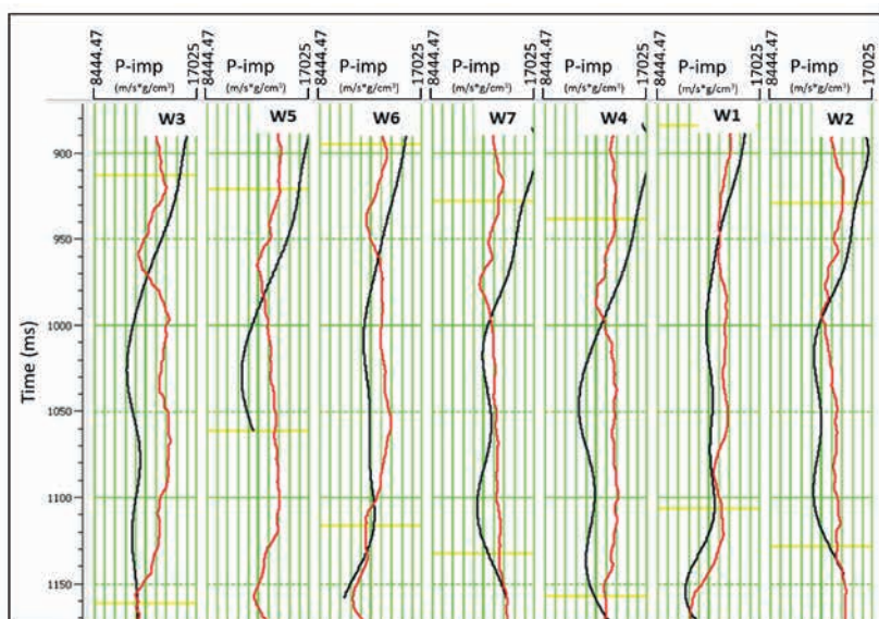
Figure 2 Match between the modelled impedance log and actual filtered impedance log using multi-attribute regression. Black curve represents the filtered impedance log and red curve represents the modelled impedance curve. Analysis window is marked by yellow bar. Poor correlation coefficient of 0.4 is observed.
