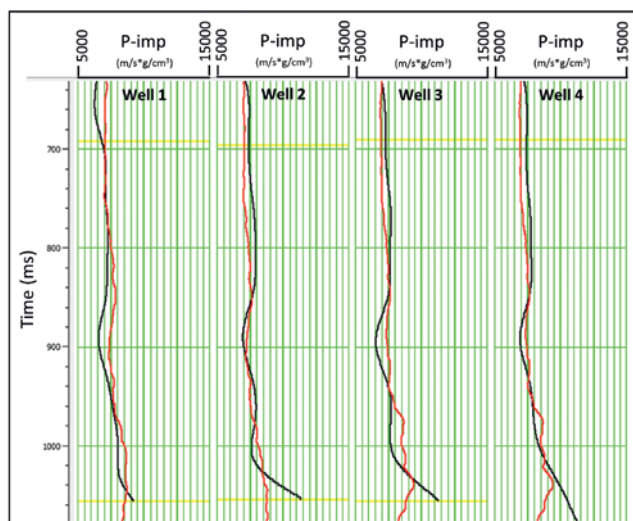
Figure 8 Match between the modelled impedance log and actual filtered impedance log using multi-attribute regression. Black curve represents the filtered impedance log and red curve represents the modelled impedance curve. Analysis window is marked by yellow bar. Poor correlation coefficient of 0.7 is observed.
