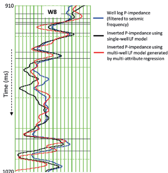
Figure 7 Match at the blind well between the actual impedance logs (blue curve), inverted impedance using single well low-frequency model (black curve) and the inverted impedance using the low-frequency model based on the proposed approach (red curve).
