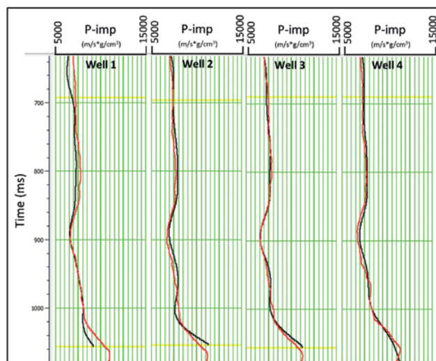
Figure 9 Match between the modelled impedance log and actual filtered impedance log using multi-attribute training network after including a single well low-frequency model as one of the inputs. Black curve represents the filtered impedance log and red curve represents the modelled impedance curve. Analysis window is marked by yellow bar. Correlation coefficient improves significantly to 0.95.
