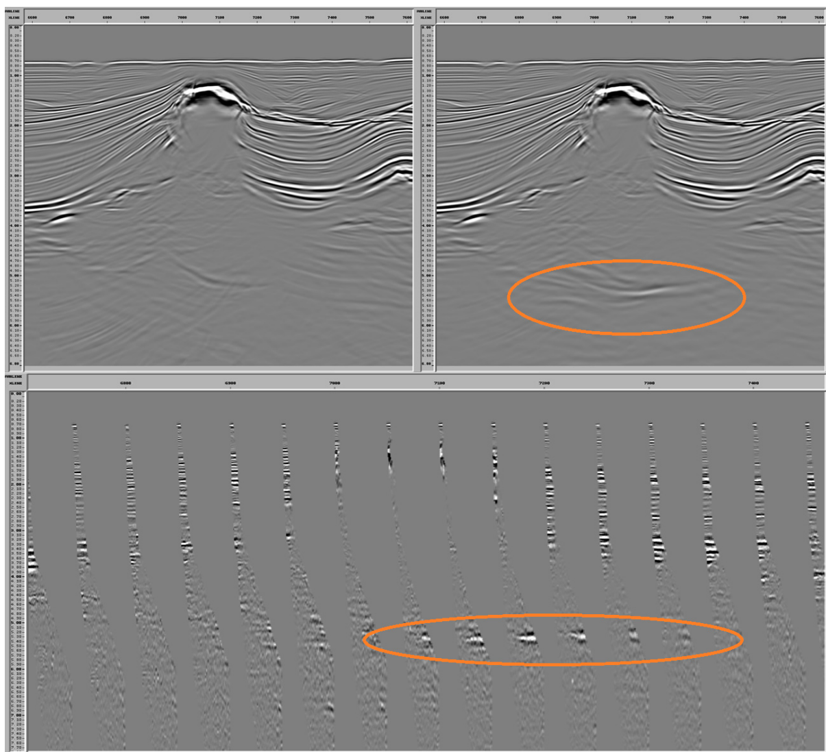
Figure 4 (upper left) Beam PSDM result for 0.3 – 6.0 km offset, (upper right) Beam PSDM result for 0.3 – 11.9 km offset, (lower) Beam PSDM 0.3 – 11.9 km image gathers after NMO correction and 15-45° angle mute applied. Note the spatially-variable contribution of very long offset reflection events to both image gathers and stacks.
