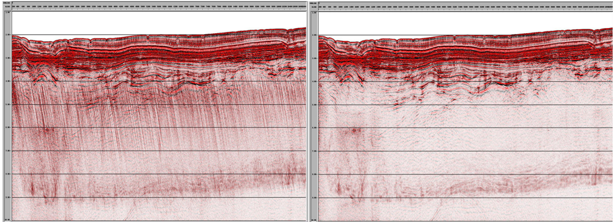
Figure 3 Brute stacks before (left) and after (right) separation of simultaneous shot gathers. The residual energy in the right panel is primarily far offset noise that has not yet been muted off.
