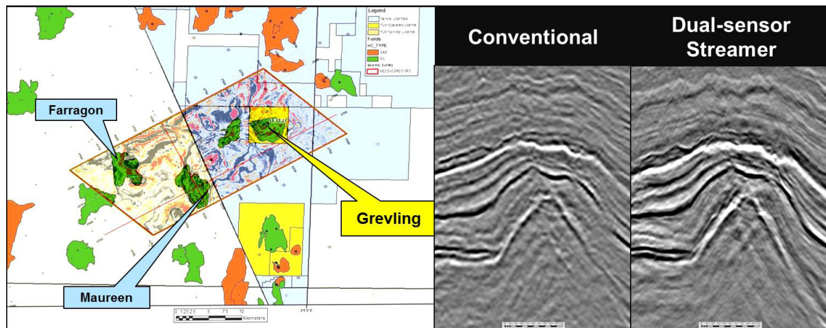
Figure 3 The left hand-side represents the location of the MultiClient survey over few North Sea fields including the Faragon and Grievling fields. The right hand-side panel shows the comparison between the conventional seismic and the dual-sensor seismic over the Upper Jurassic Grevling field. The dual-sensor streamer seismic exhibits a significant increase bandwidth.
