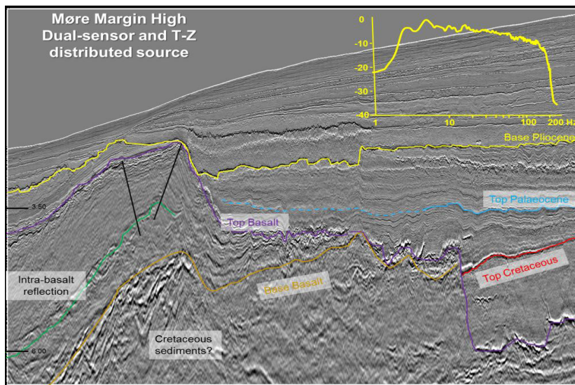
Figure 2 the figure represents a portion of a seismic line (Møre Marginal High, Norway) acquired with a dual-sensor streamer and depth-time distributed source-arrays. The amplitude (log scale) has been computed in the Pliocene interval and shows a frequency bandwidth from 2.5/3Hz up to 180 Hz. Previously not seen, intra-basalt reflections are now visible with this new dataset with also a good signal to noise ratio.
