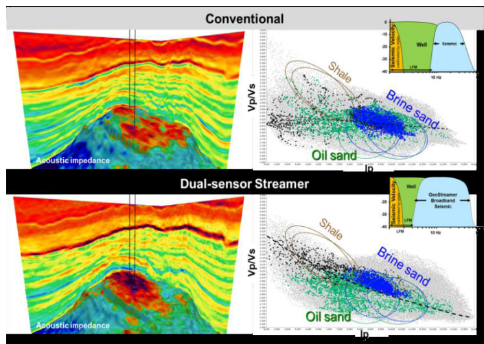
Figure 4 The figure illustrates the results of the inversion over the conventional and the dual-sensor datasets. Red color is low acoustic impedance and blue is high acoustic impedance. The results of the dual-sensor acoustic impedance match very well with the structure in comparison of the conventional seismic results. Also, when the seismic driven elastic attributes are projected to the rock physics template, the match between the rock physics and the elastic attributes is very good using the dual-sensor streamer results.
